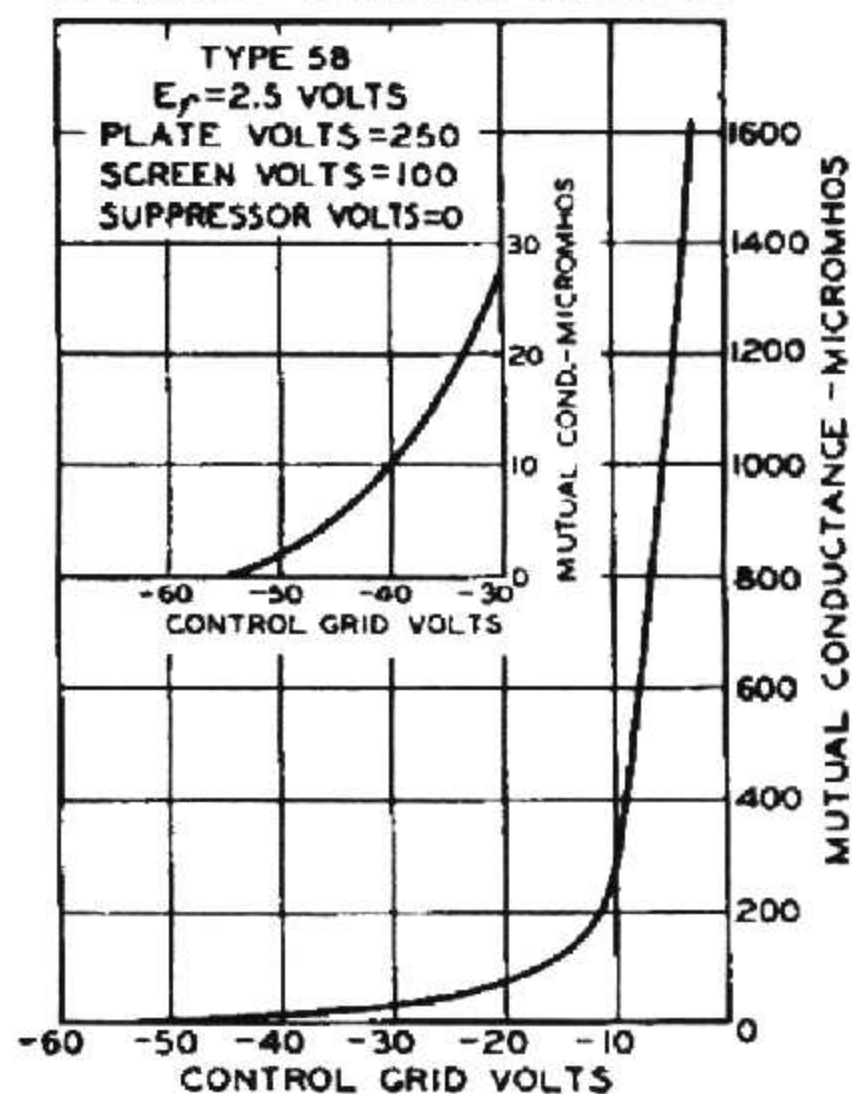
AVERAGE CHARACTERISTICS
