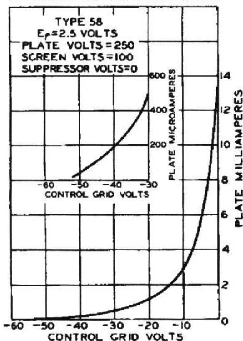
AVERAGE CHARACTERISTICS
